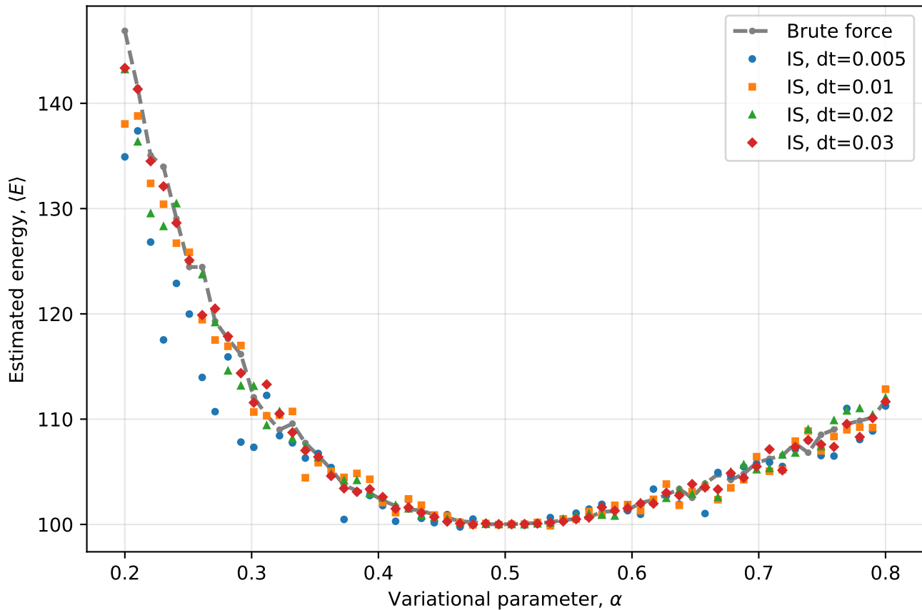
E(\alpha) for N=100 , D=2
