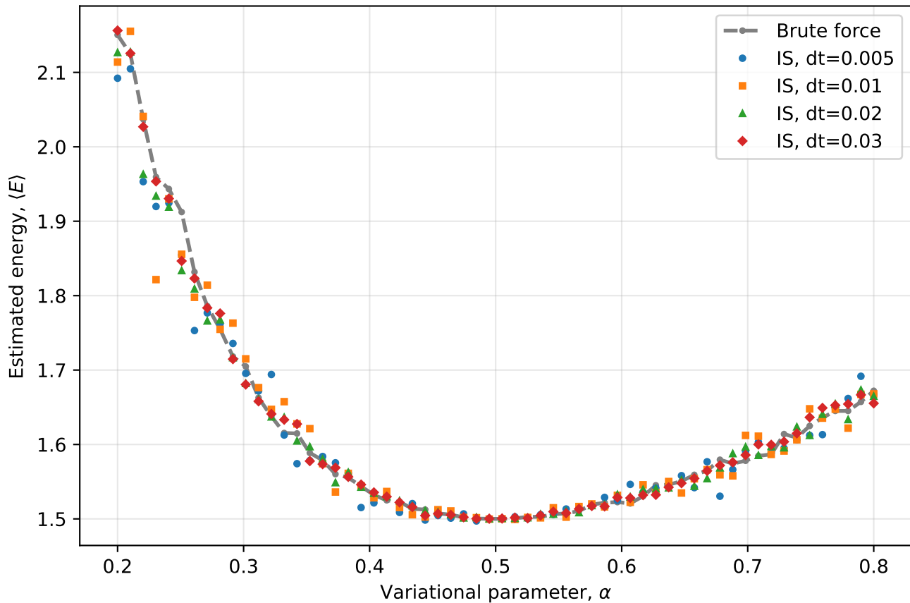
E(\alpha) for N=1 , D=3
