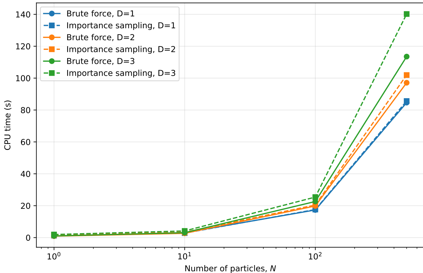
CPU time vs N : brute force vs importance sampling
