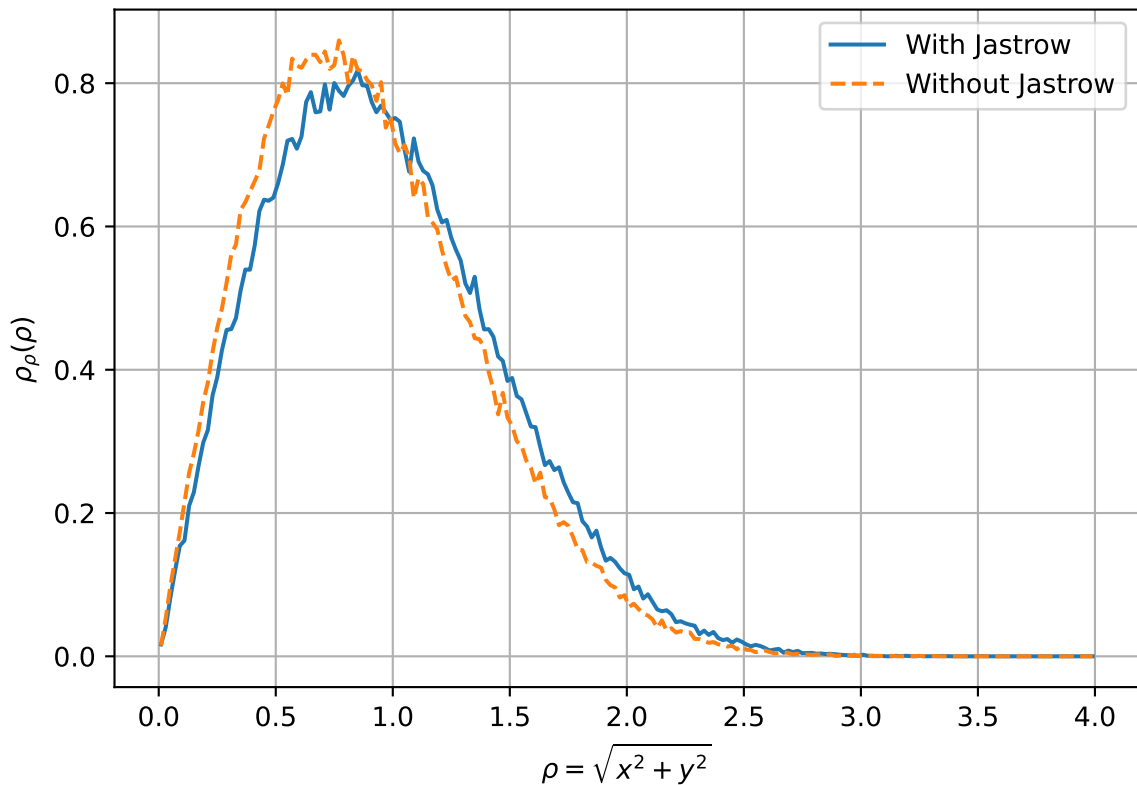
One-body density in transverse plane: N = 100 , D = 3
