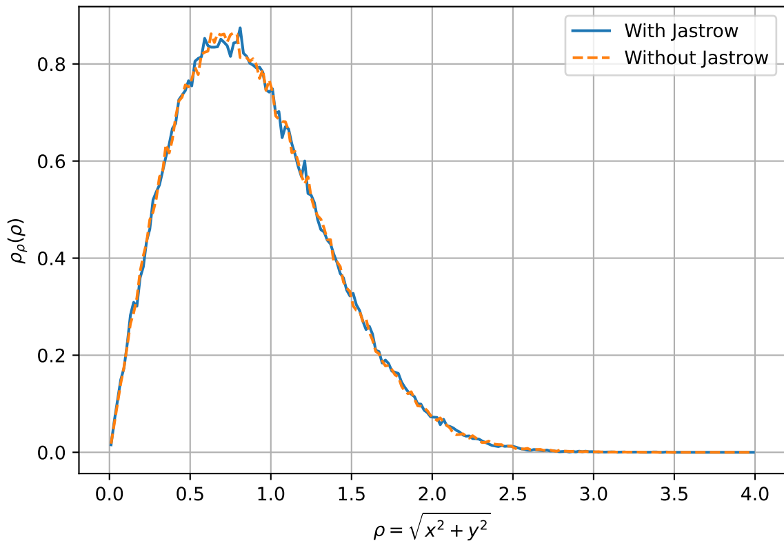
One-body density in transverse plane: N = 10 , D = 3
