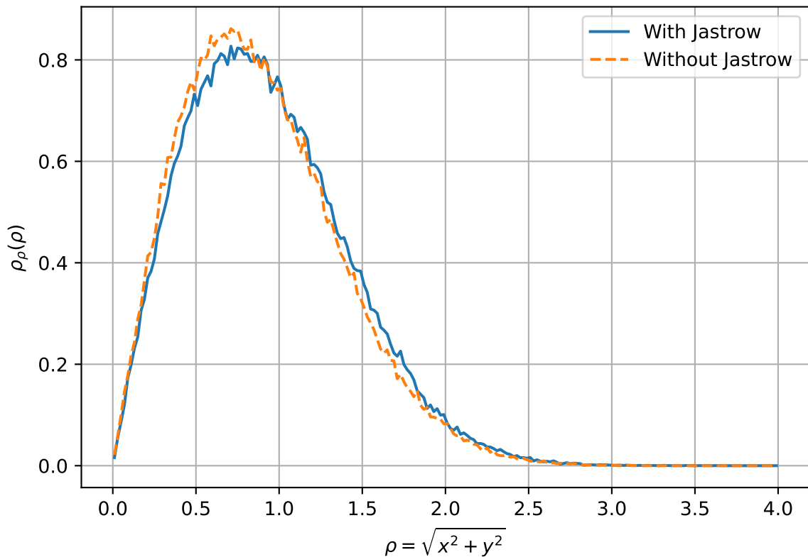
One-body density in transverse plane: N = 50 , D = 3
