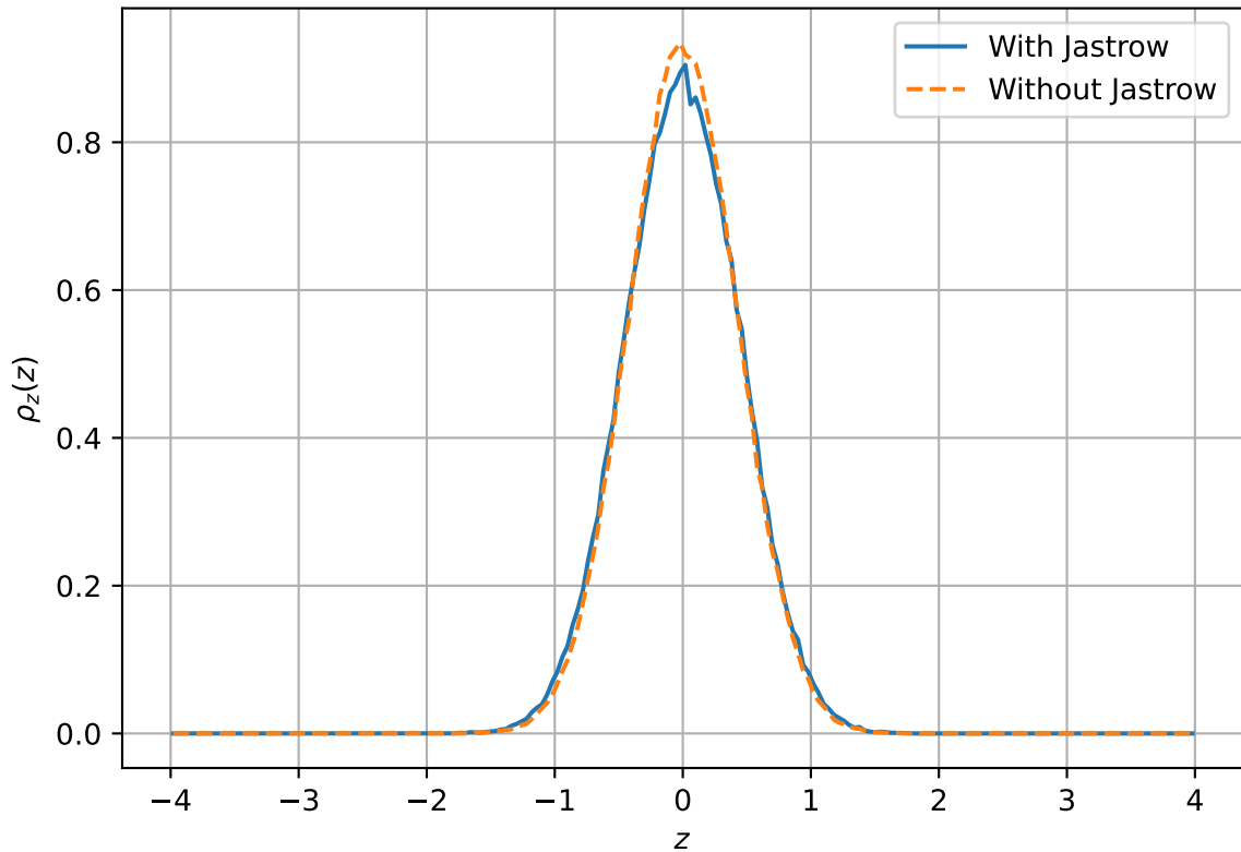
One-body density along z : N = 100 , D = 3
