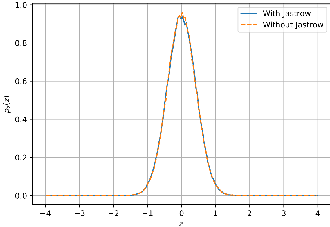
One-body density along z : N = 10 , D = 3
