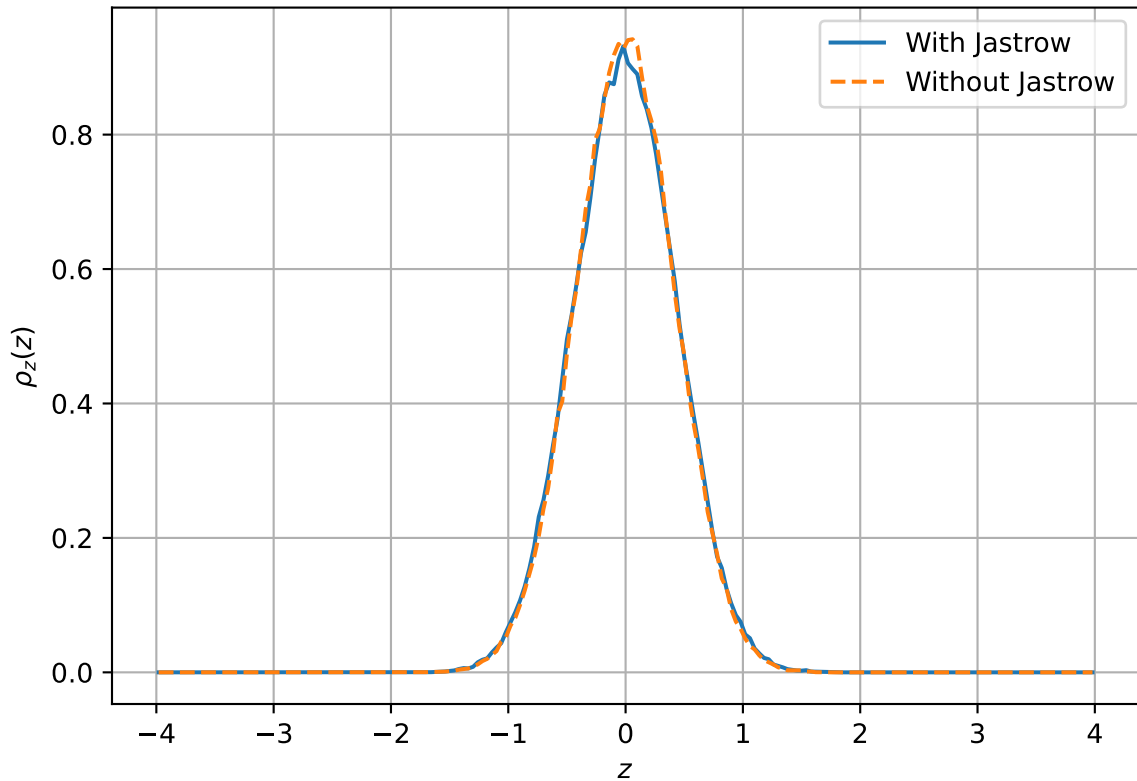
One-body density along z : N = 50 , D = 3
