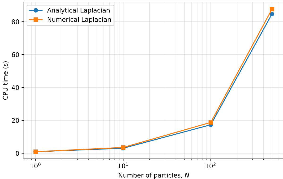
CPU time vs number of particles in 1D
