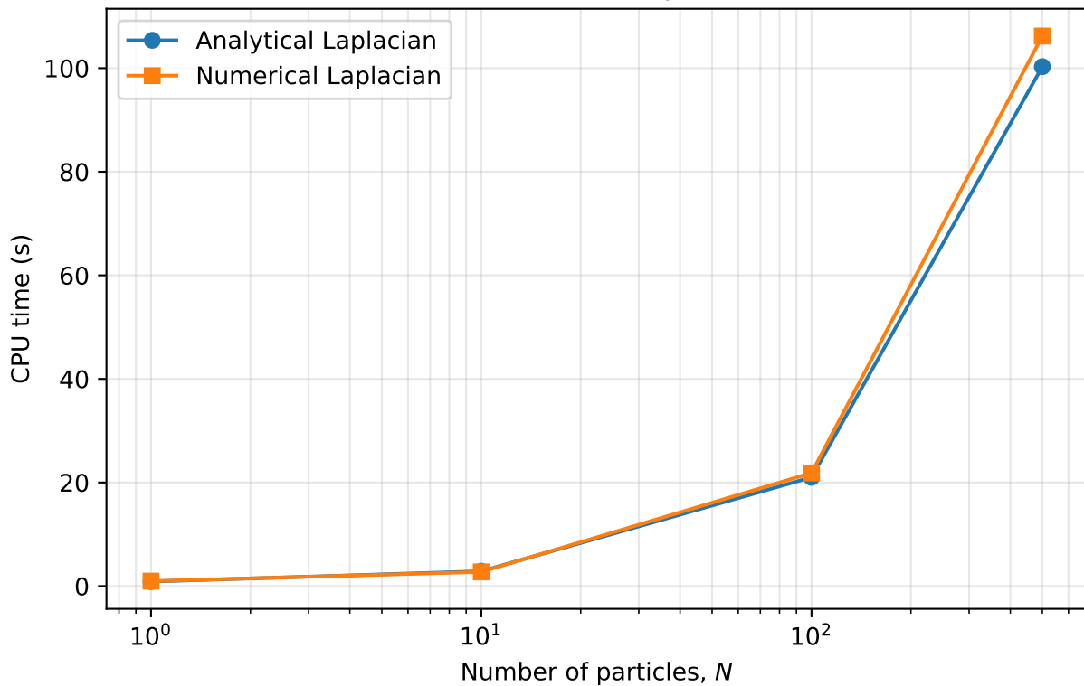
CPU time vs number of particles in 2D
