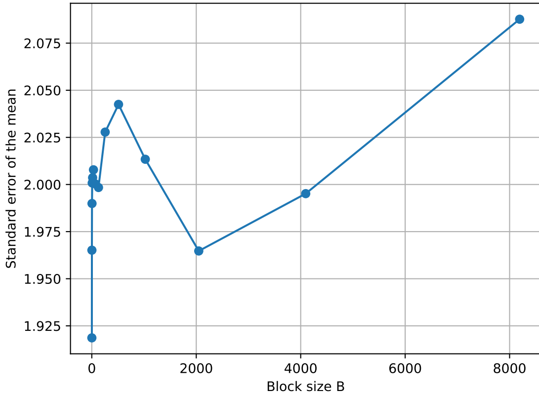
Standard error of the mean vs block size for N=1 , \beta=1.0 , a=0.0
