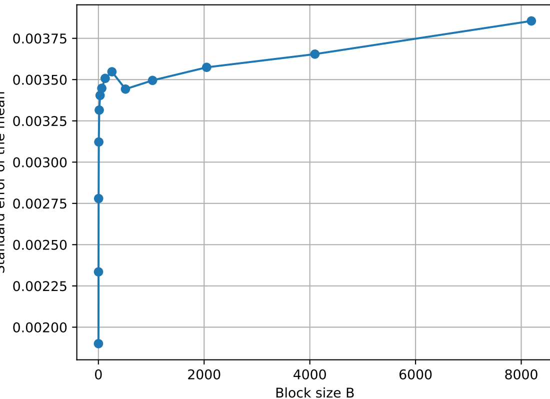
Standard error of the mean vs block size for N=2 , \beta=2.82843 , \alpha=0.0
