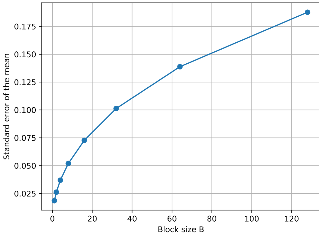
Standard error of the mean vs block size for N=10 , \beta=2.82843 , a=1.0
