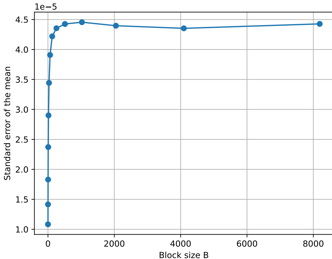
Standard error of the mean vs block size for N=10 , \beta=1.0 , a=0.0
