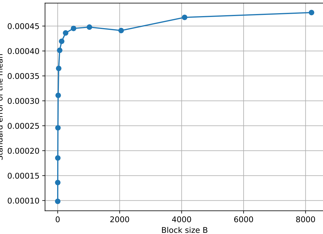
Standard error of the mean vs block size for N=10 , \beta=2.82843 , a=0.0
