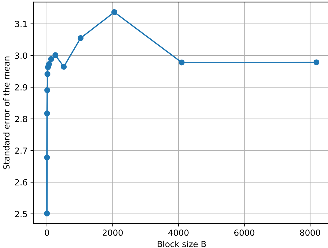
Standard error of the mean vs block size for N=2 , \beta=1.0 , a=0.0
