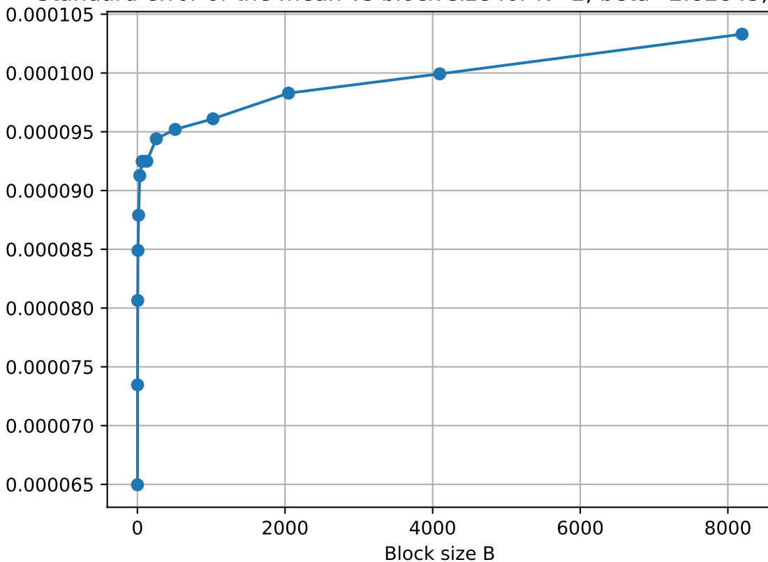
Standard error of the mean vs block size for N=2 , \beta=2.82843 , a=0.0
