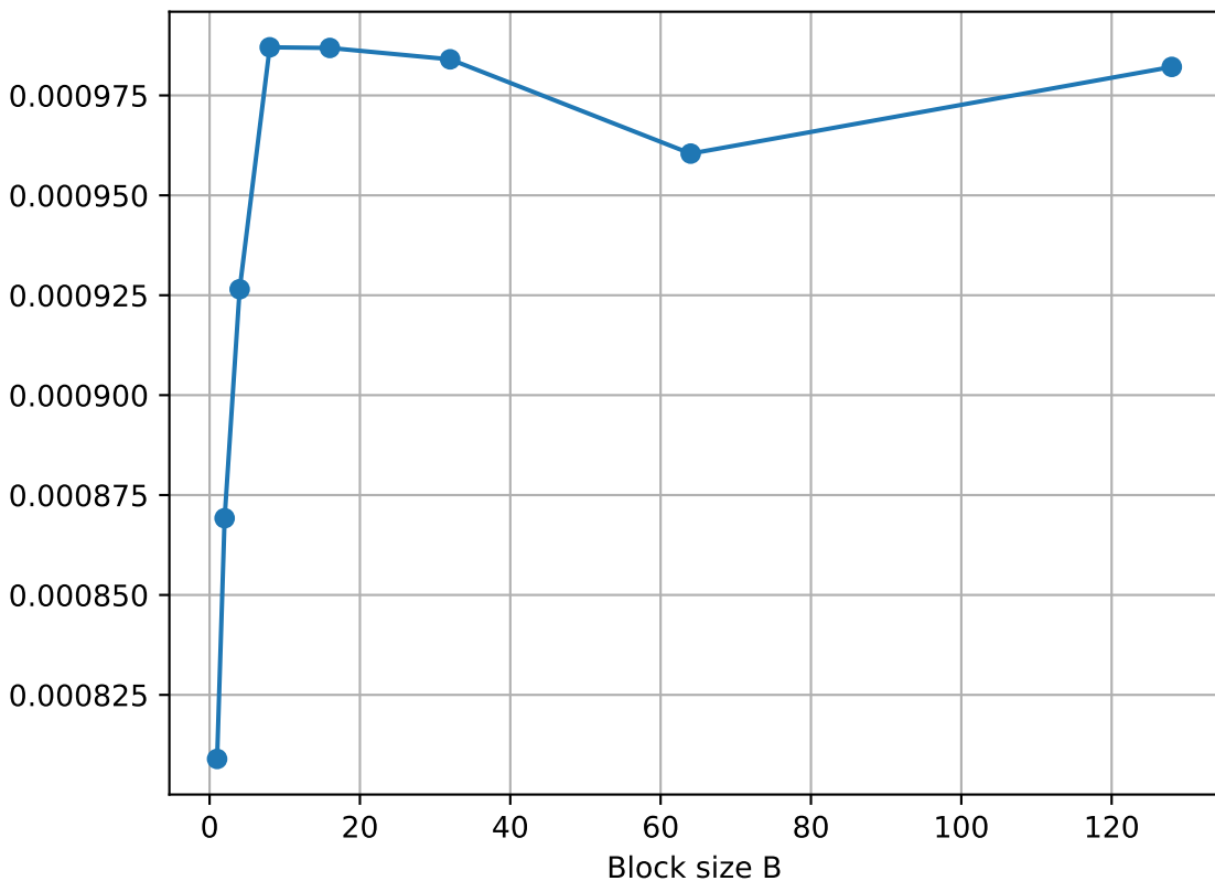
Standard error of the mean vs block size for N=2 , \beta=2.82843 , \alpha=0.0043
