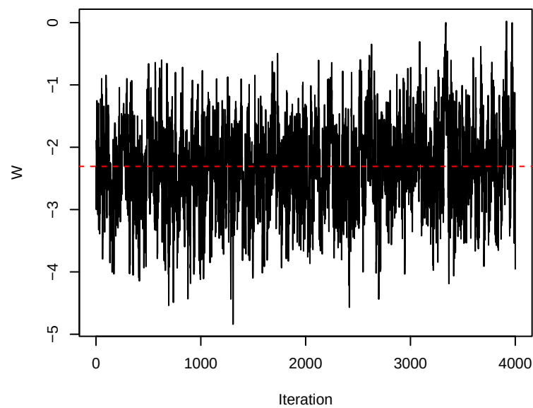
mail-drop_u01b-cancomefolder (d=1, mean=-2.307)
