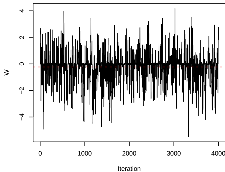
toolbar_move (d=1, mean=-0.234)
