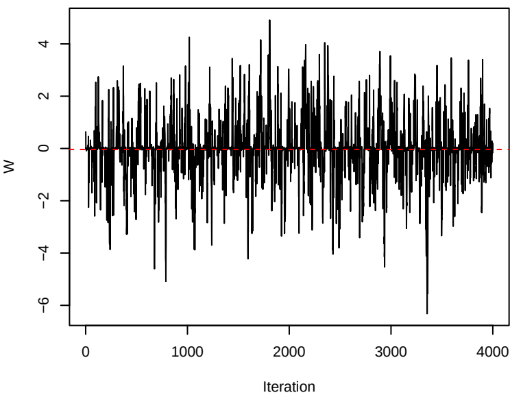
mail-viewed_u23-item305 (d=1, mean=1.78)
