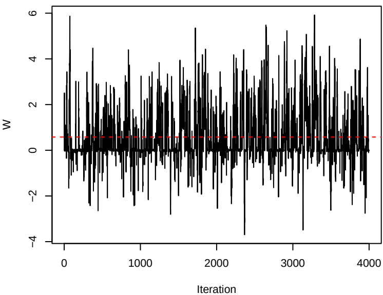
restart (d=1, mean=0.495)
