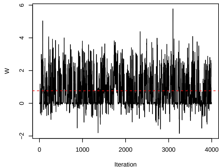
folder-unfolded_u01a-partyfolder (d=1, mean=0.766)
