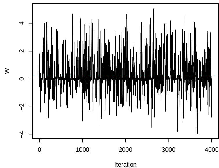
mail-drop_u01a-mymails (d=1, mean=0.294)
