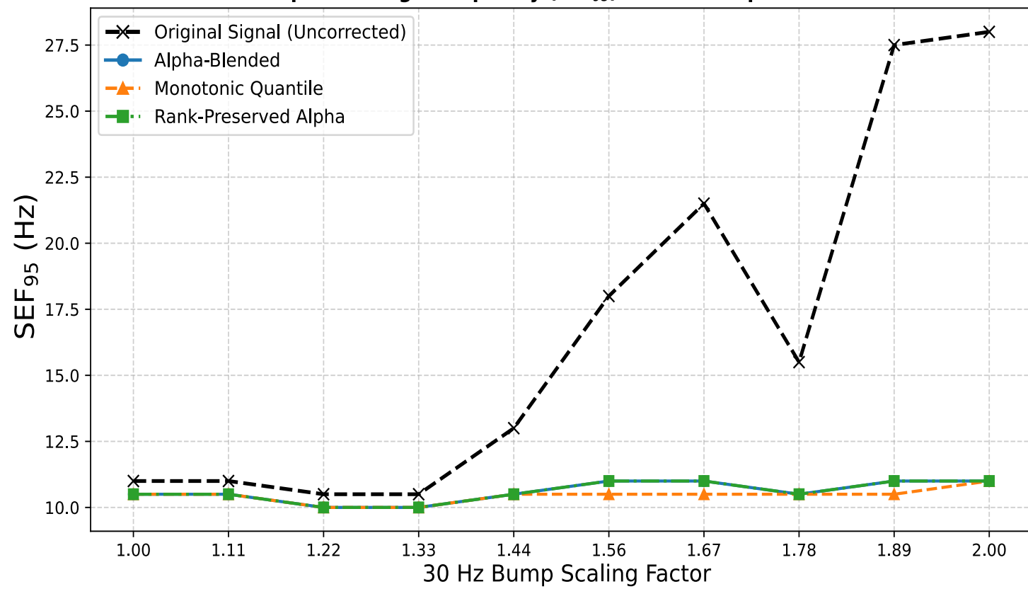
Spectral Edge Frequency ( \text{SEF}_{95} ) across Bump Factors
