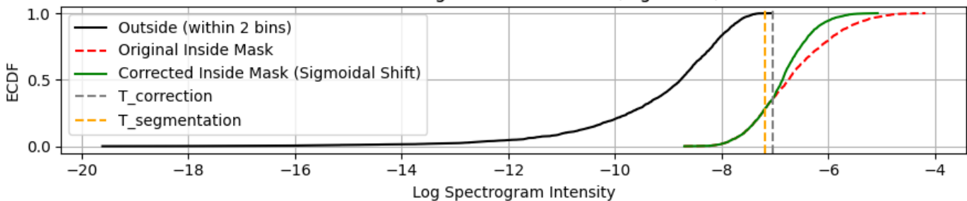
ECDF Matching &amp; Transformation (Sigmoidal)
