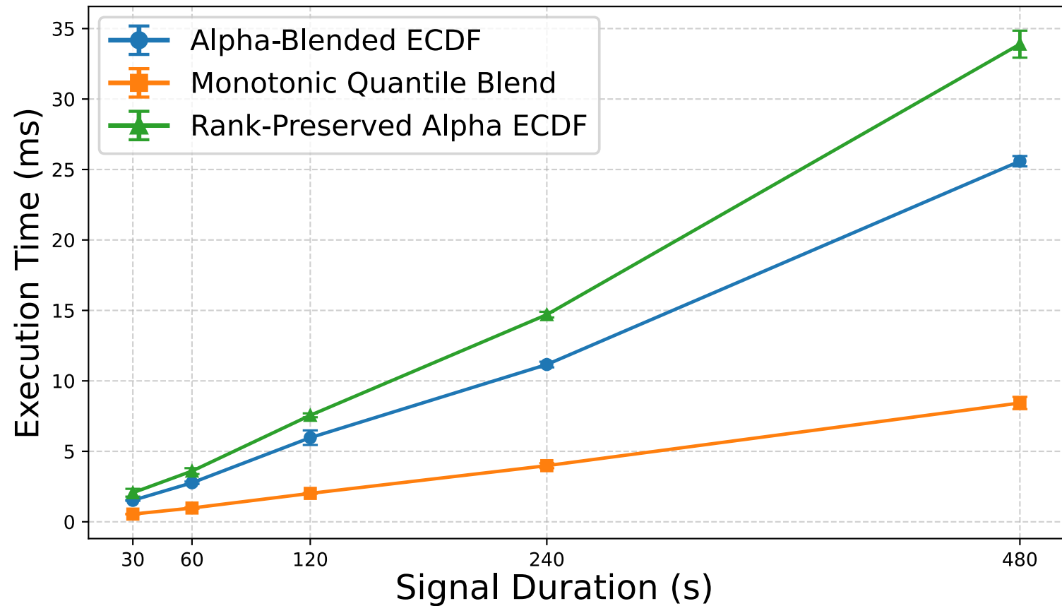
Execution Time Trend vs. Signal Duration
