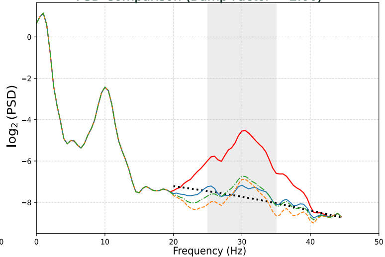
PSD Comparison (Bump Factor = 2.00)
