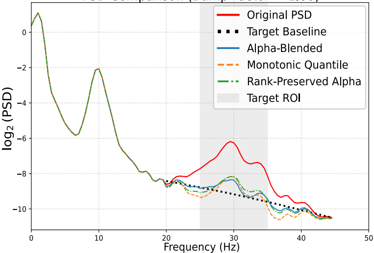
PSD Comparison (Bump Factor = 1.00)
