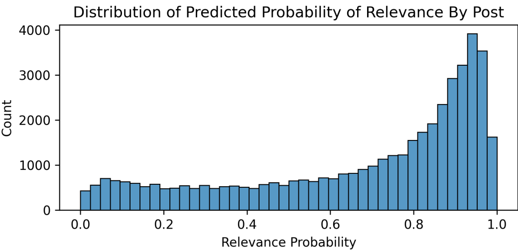
Figure 2: Distribution of LR-predicted relevance probability
