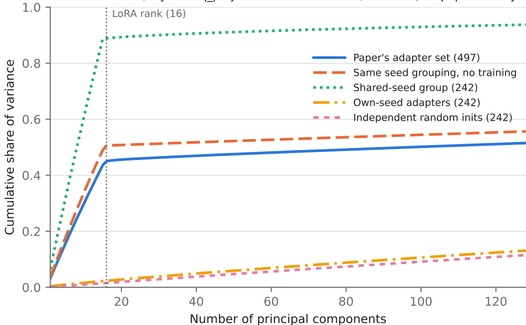
LoRA A matrices, layer 16 q_proj: stacked rank vectors, centred (the paper's analysis)
