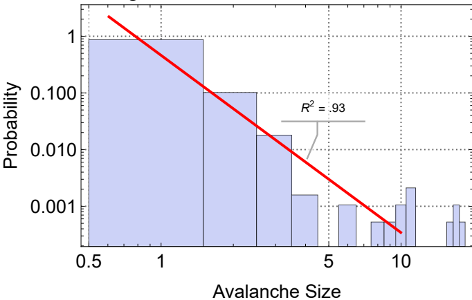
Congestion avalanche size distribution
