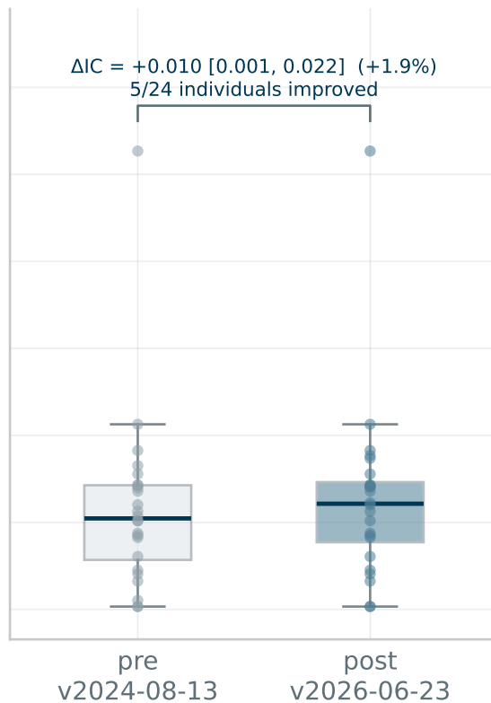
NFKB1 (n = 24)
