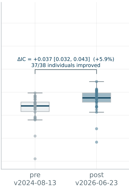
APDS1 (n = 38)
