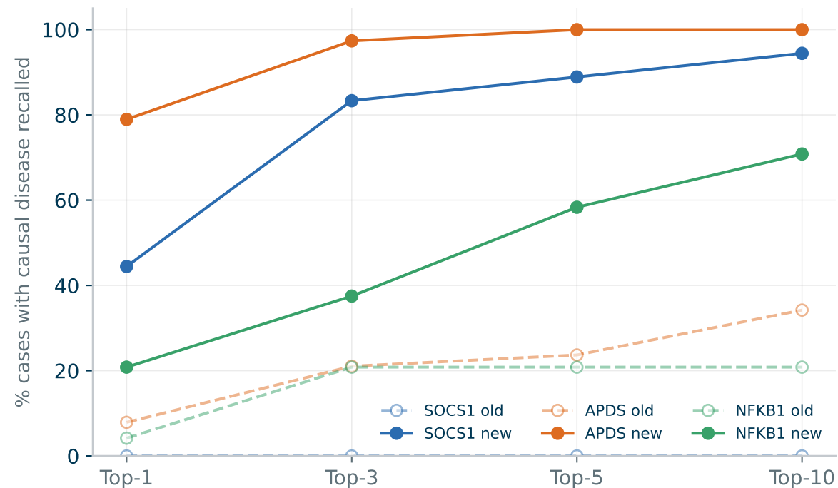
Top-k recall: old (dashed) vs new (solid)
