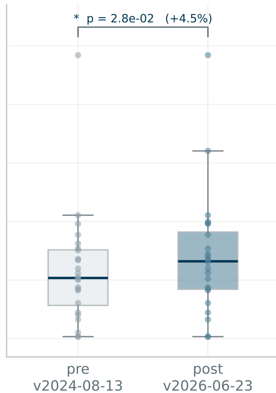
NFKB1 (n = 24)
