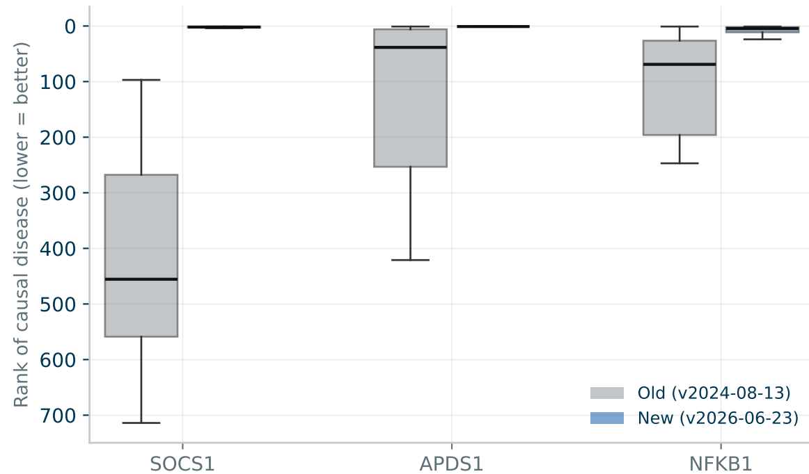
LIRICAL ranking: old vs new HPO
