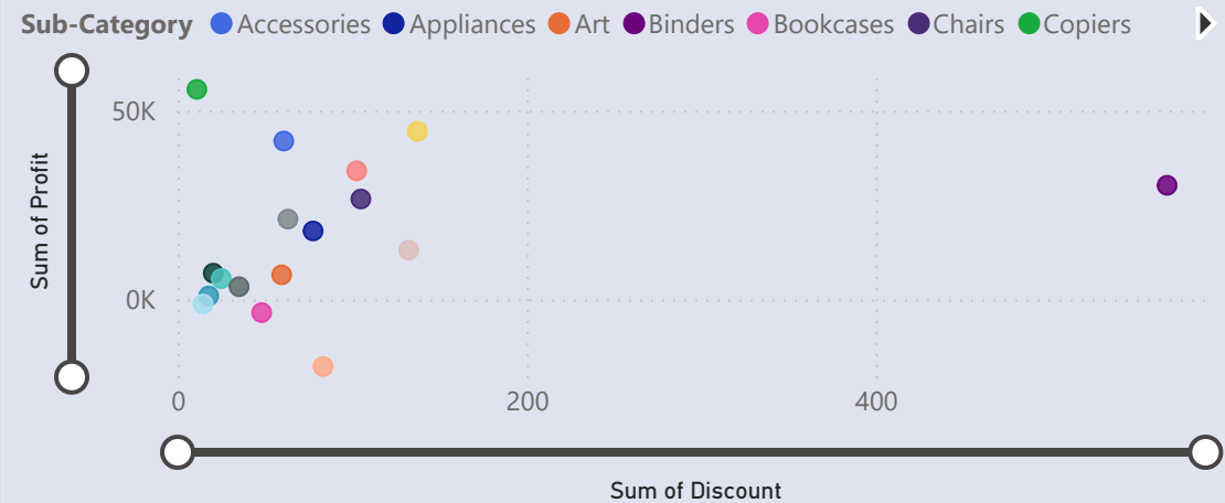
Profit vs Discount Scatterplot
