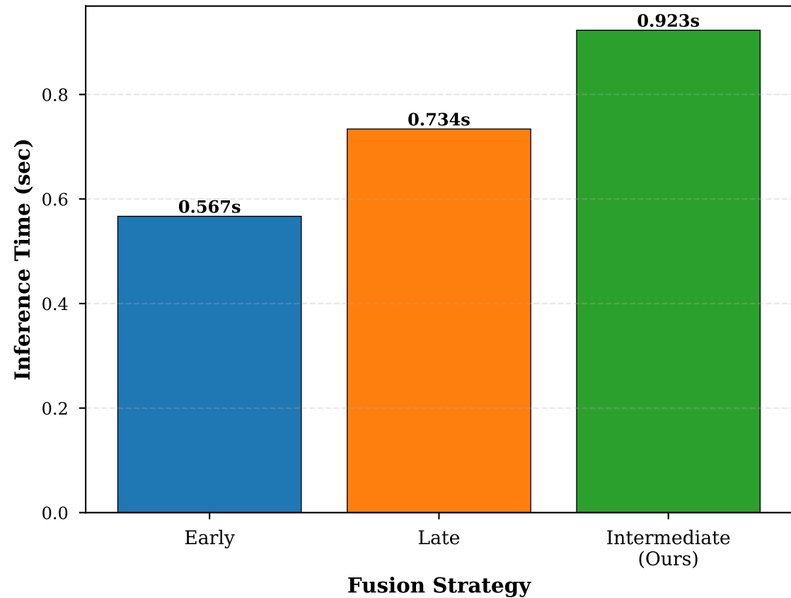
Computational Cost
