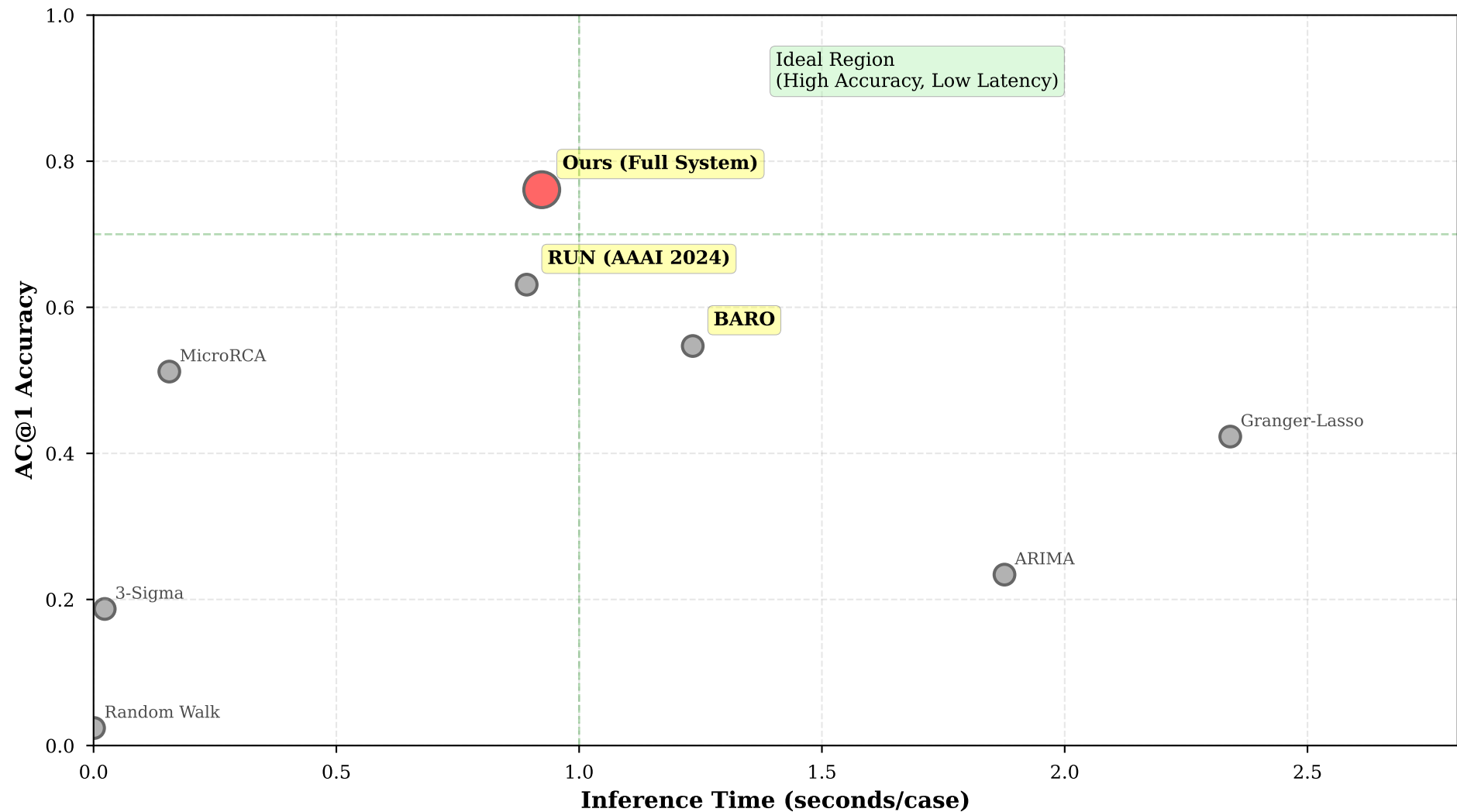
Accuracy vs Inference Time Trade-off
