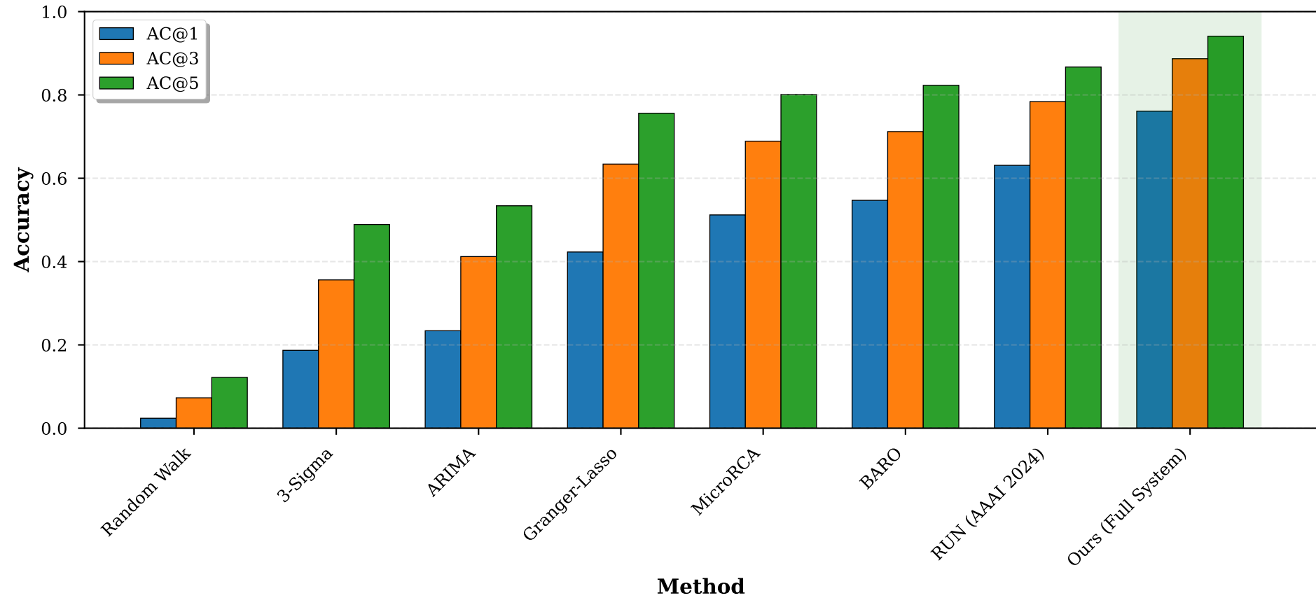
Root Cause Analysis Performance: Baseline Comparison
