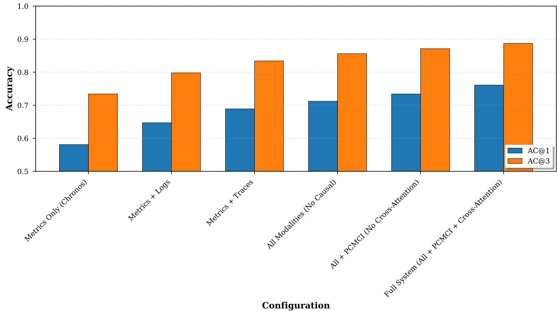
Ablation Study: Incremental Component Gains
