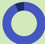
Python
