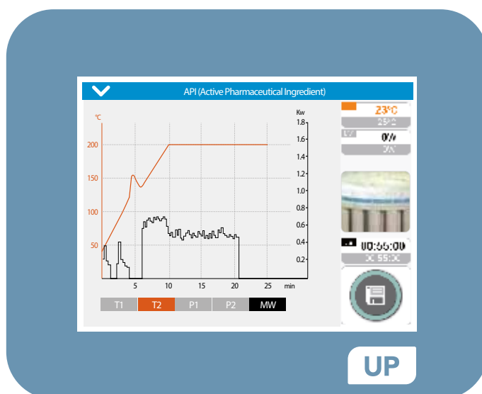
easyTEMP temperature control of an exothermic reaction during the digestion of an API with \text{HNO}_3 and \text{HCl} in the SK-15 rotor
