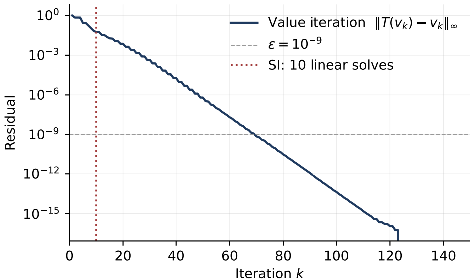
Convergence of value iteration vs. strategy iteration
