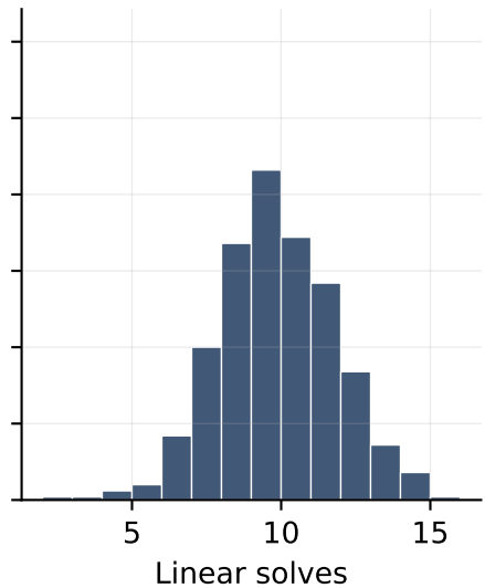
SI iteration counts over 500 random initial policies
