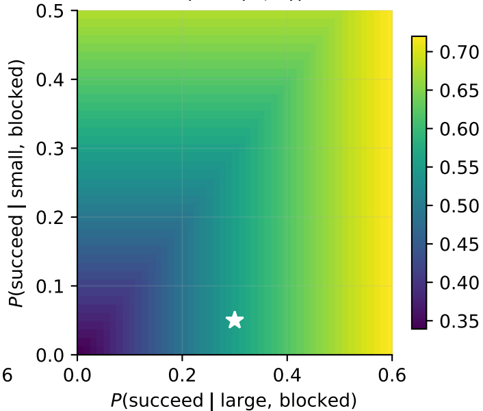
W(\text{Max}(H, 6))
