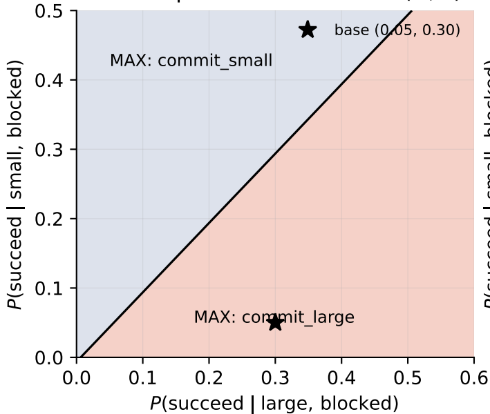
MAX's optimal action at \text{Max}(H, 6)
