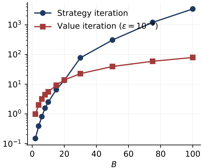
Solve time vs. B
