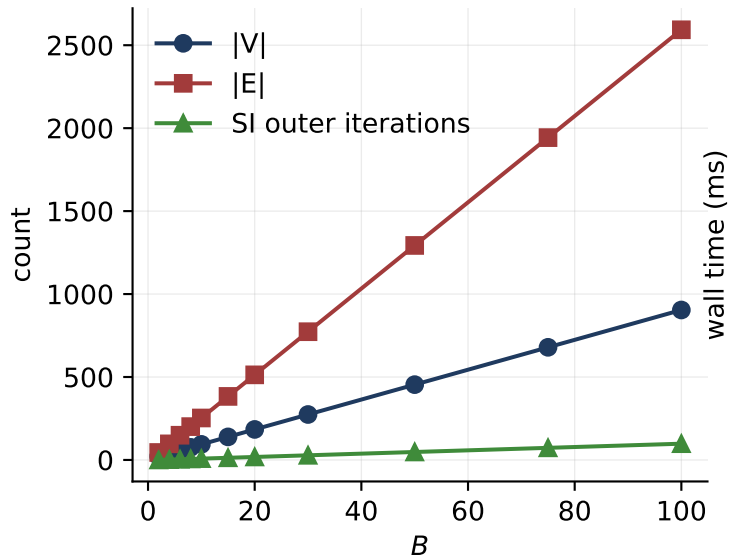
Graph size and SI outer iterations vs. B
