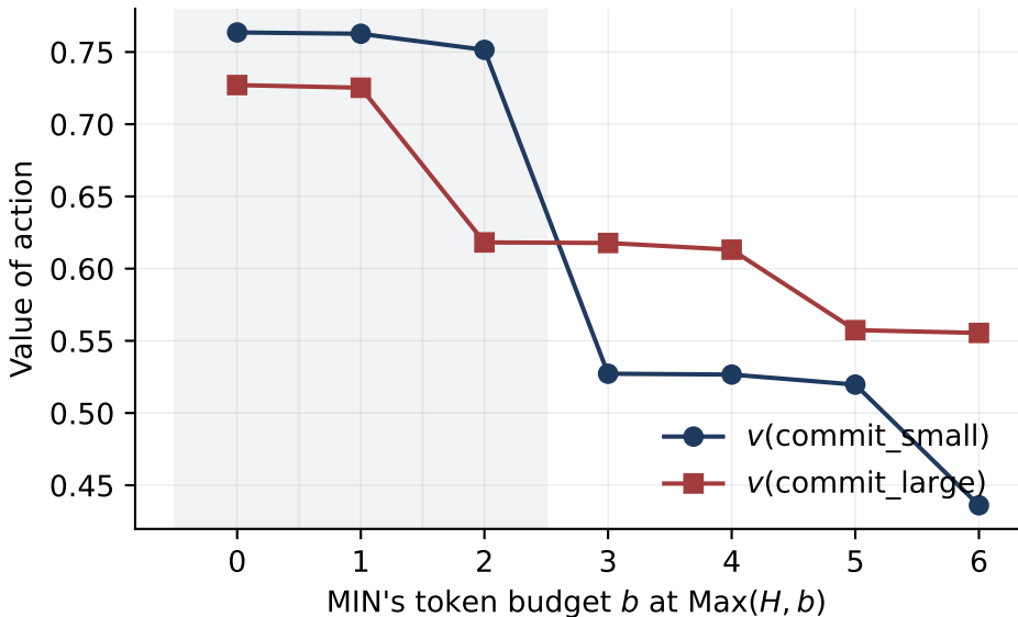
Optimal MAX action by MIN's budget (shaded: MAX prefers small)
