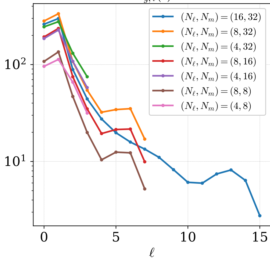
W_{g,i}(\ell)
