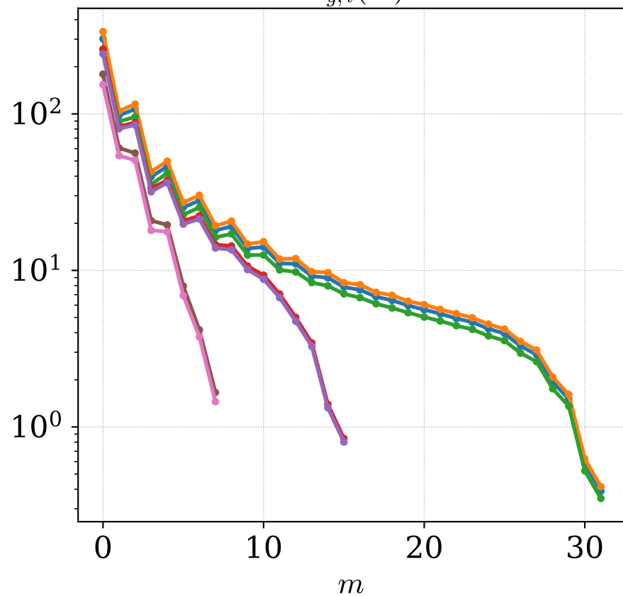
W_{g,i}(m)
