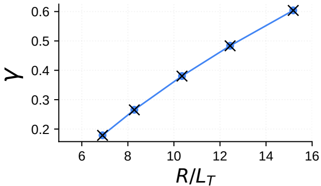
(b) \gamma vs R/L_T
