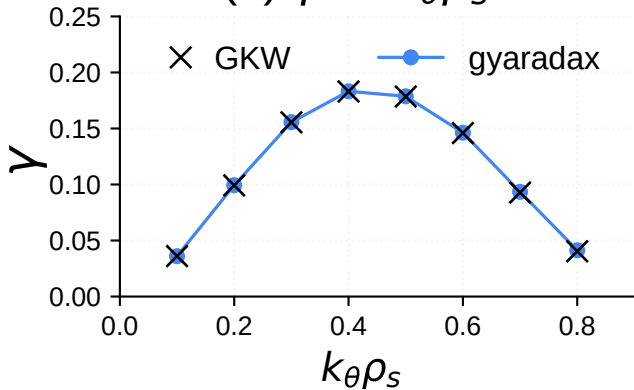
(a) \gamma vs k_{\theta}\rho_s
