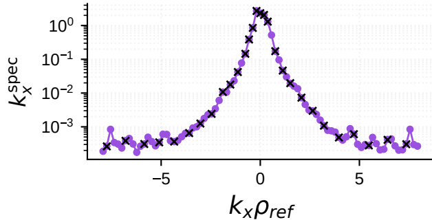
k_x spectrum
