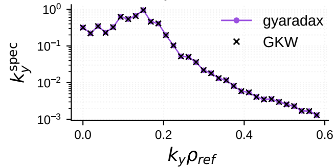
k_y spectrum
