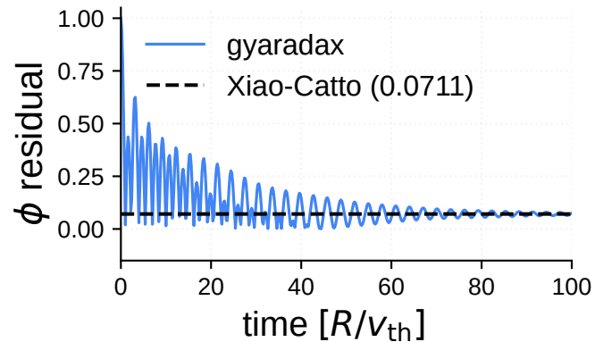
(a) zonal flow residual
