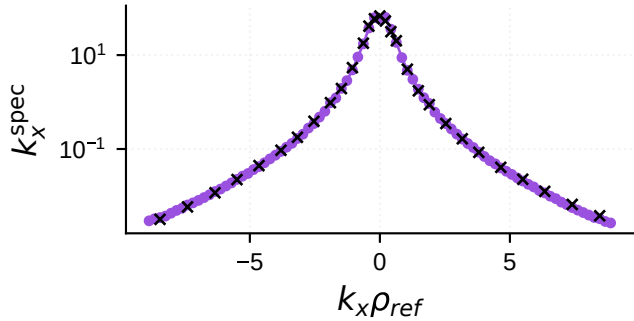
k_x spectrum
