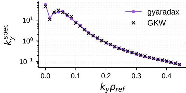
k_y spectrum
