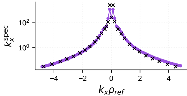
k_x spectrum
