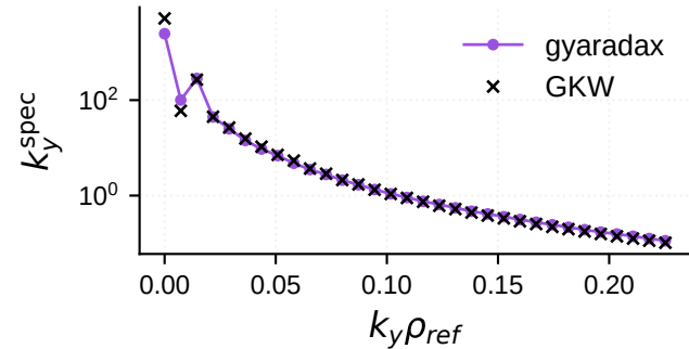
k_y spectrum
