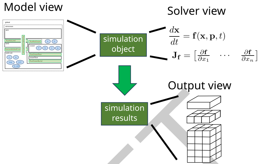
Figure 2: PALEO provides three views on model simulation and results, with appropriate abstractions for (i) implementing Reactions that generate biogeochemical transformations and transport between biogeochemical reservoirs; (ii) numerical solution as an initial value problem by ODE or DAE solvers, or analysis as a dynamical system; and (iii) analysis of time-series or steady-state results
