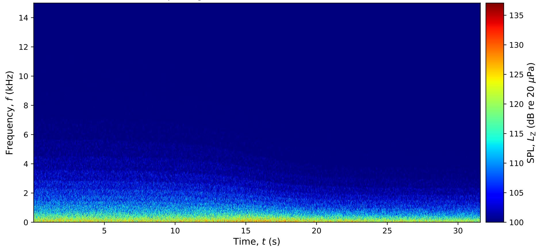
OUTPUT - Spectrogram of auralized BBN - emission - airframe
